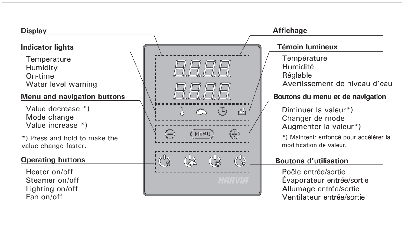
Figure 2. Control panel
