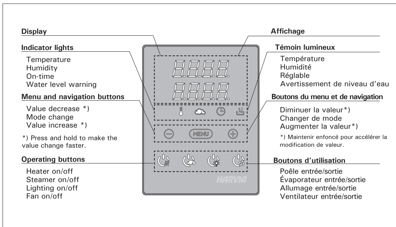
Figure 2. Control panel Figure 2. Le tableau de commande
