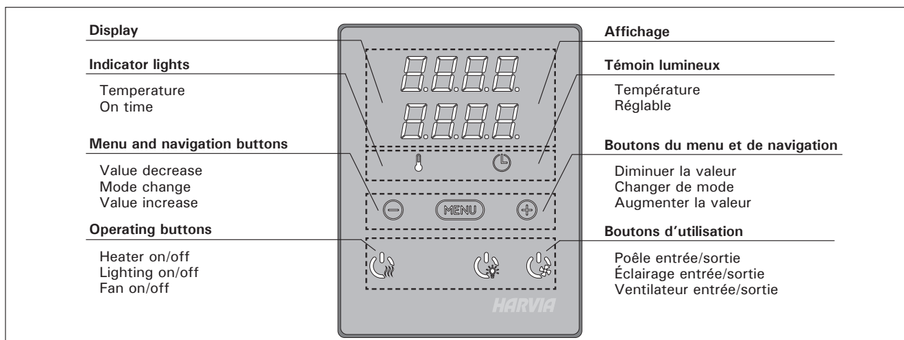
Figure 2. Control panel
