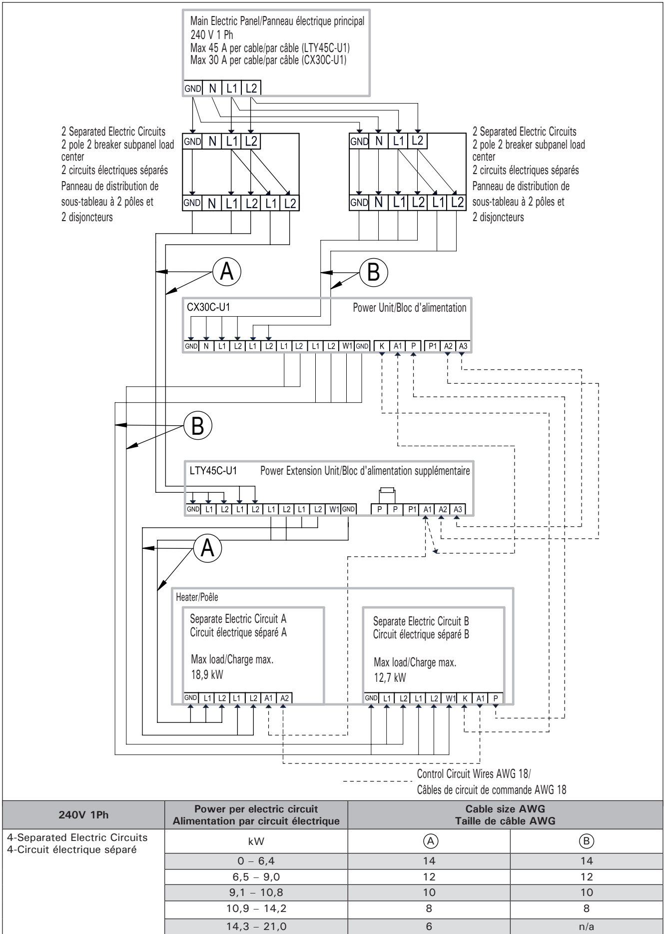
Figure 16. Connection of power extension unit LTY45C-U1 with control unit CX30C-U1 (240 V / 1 Ph) (Two separated electric circuits between power extension unit and heater). Heater with one built-in steamer units and one pair of A1/A2 terminals
